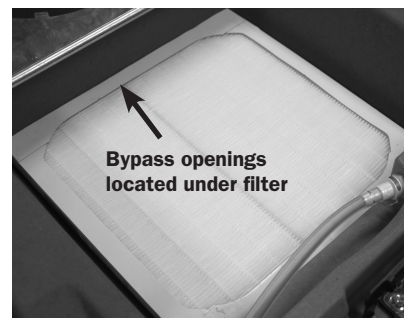
Remove filter, snap grain control cover into position shown, and replace filter.
