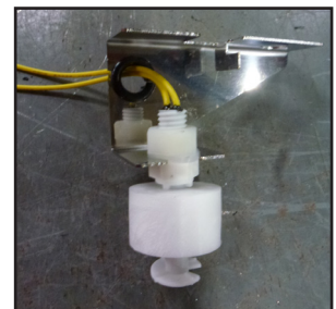
Figure 8: Picture of the float safety switch.
