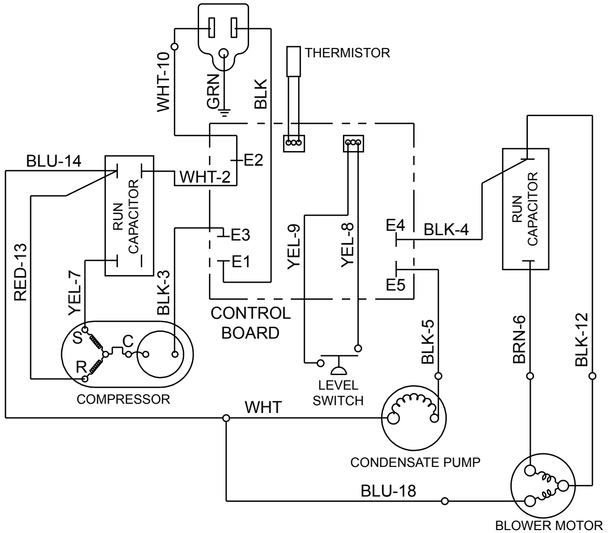
Figure 9: Wiring diagram
