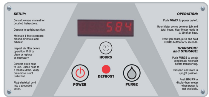
Figure 2: Phoenix R200 control board.
