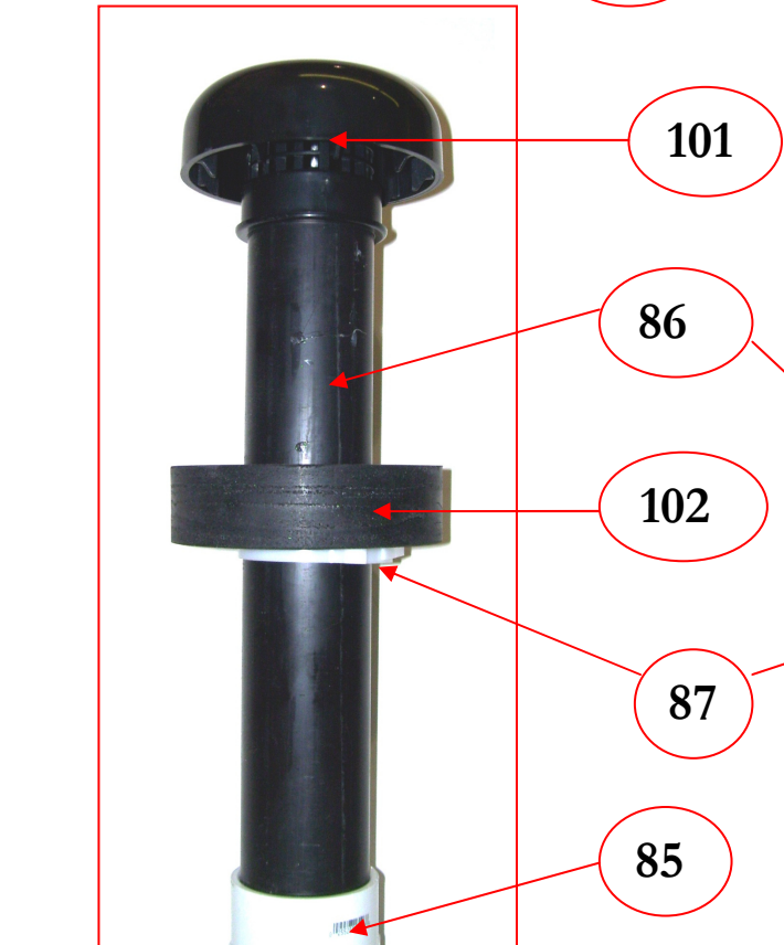
VACUUM SHUTOFF ASSEMBLY
