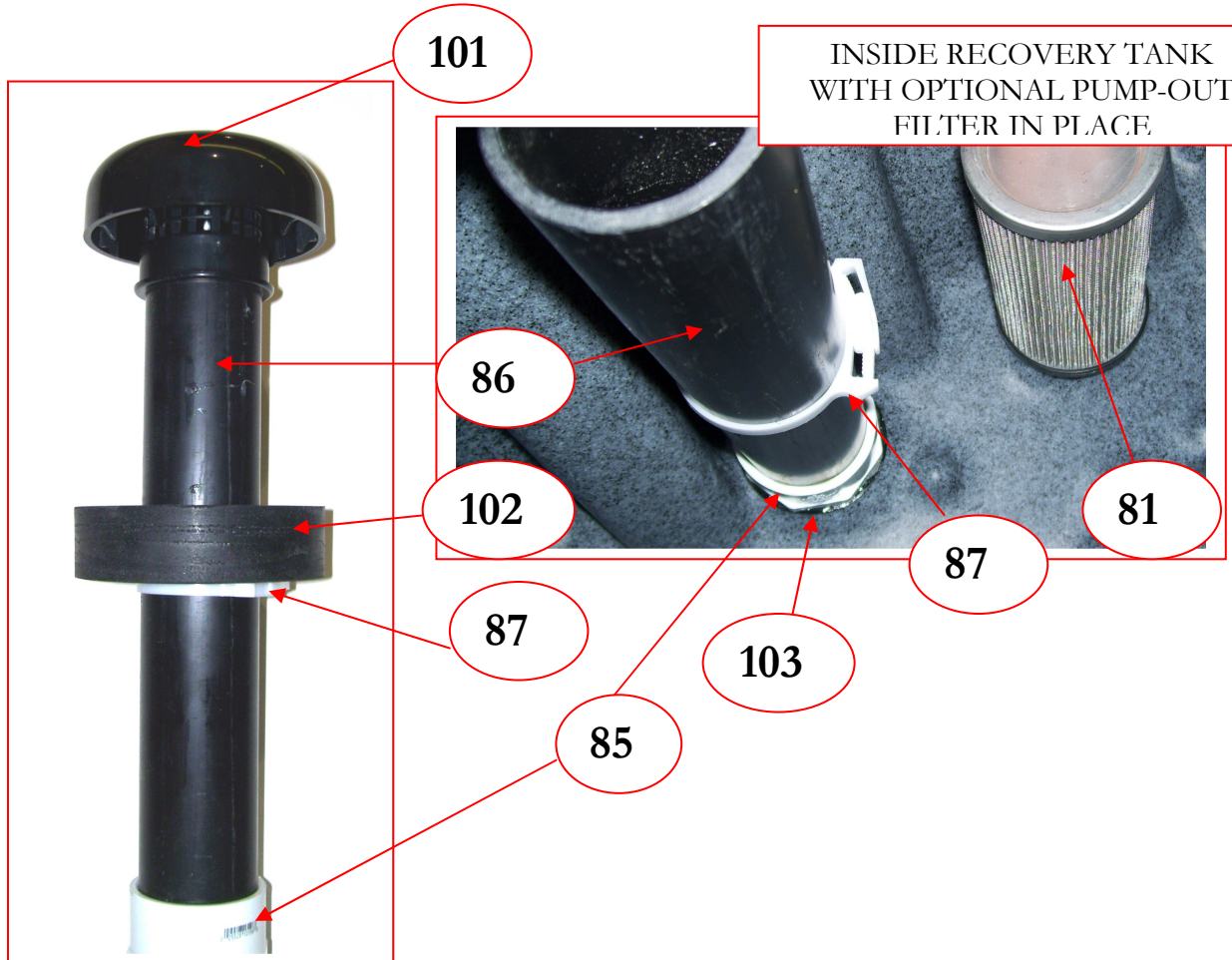
VACUUM SHUTOFF ASSEMBLY
