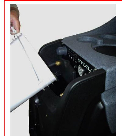
Pour 2 or 3 gallons of clean water into Solution Tank
