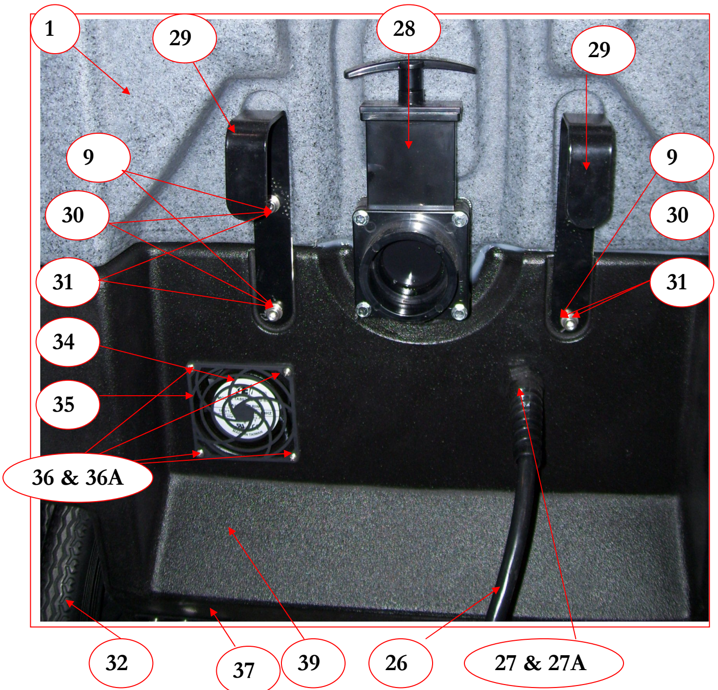
REAR VIEW – BASE, BASE SKIRT & RECOVERY TANK
